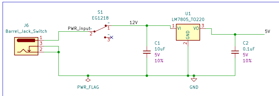
Input and 5V circuit
