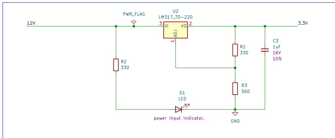
3.3V circuit
