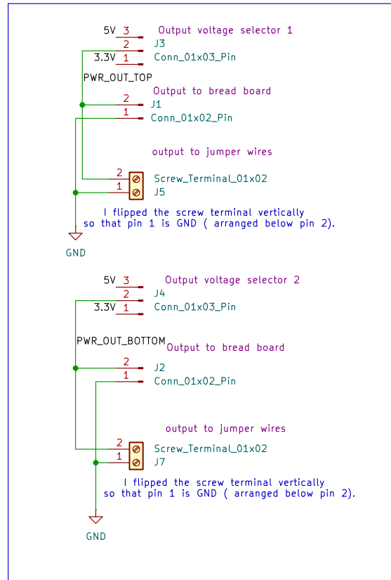
Output and Switches
